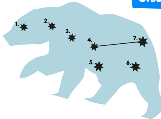
Ursa Major
